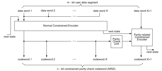
Fig. 1. Block schematic for encoding a constrained PC code in NRZI format.
