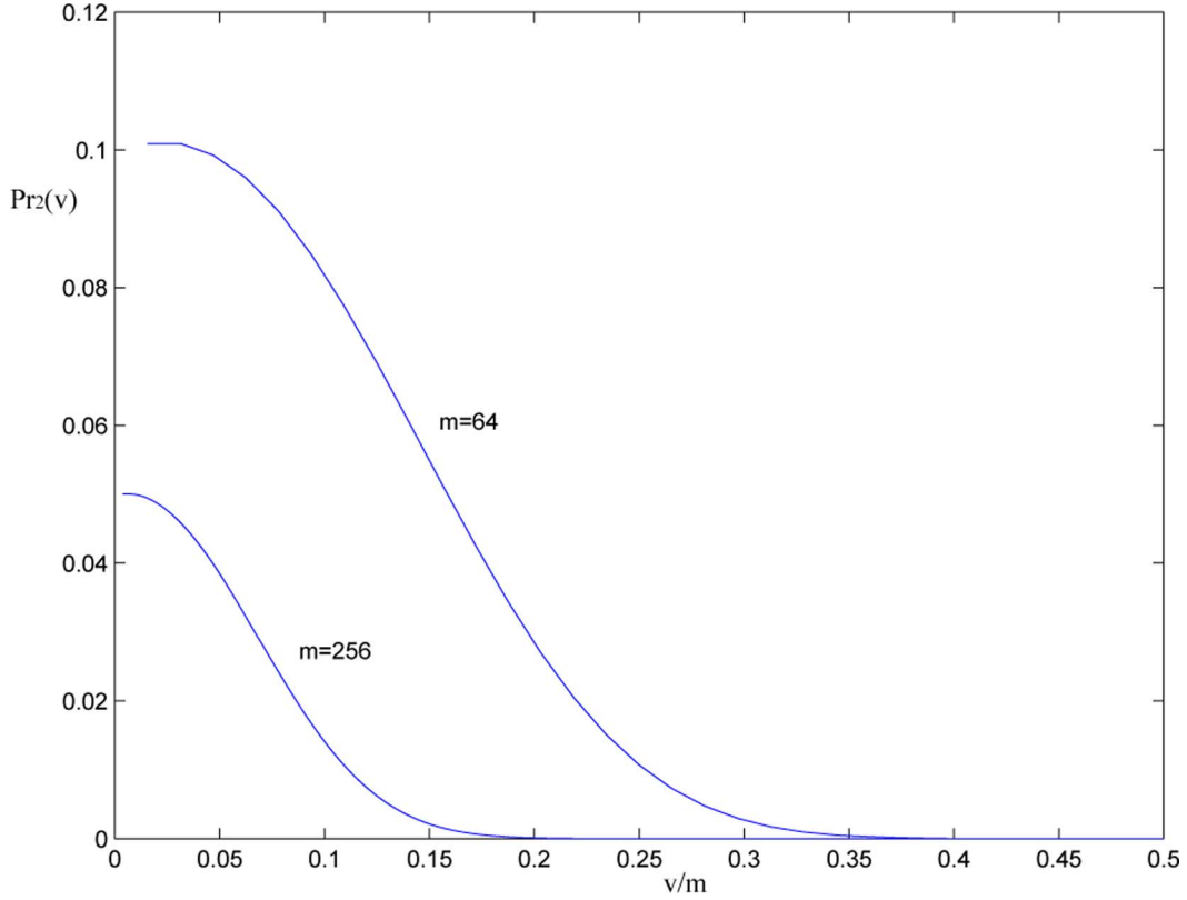
Fig. 3. Distribution Pr_2(v) of the (normalized) number, v/m , of possible balancing positions for m = 64 and m = 256 .
