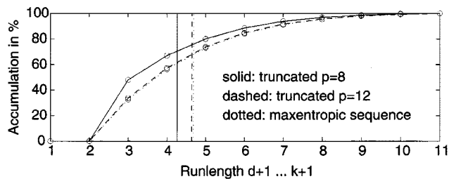
Fig. 2. Accumulated runlength distributions of two (2, 10, 15) constrained enumerative codes having a rate of 256/512 (obtained in computer simulations; solid, dashed) and the accumulated runlength distribution of the corresponding maxentropic sequence (obtained with the method developed by Kerpez et al. [9], denoted by the dotted line). The step functions indicate the corresponding average runlengths.
