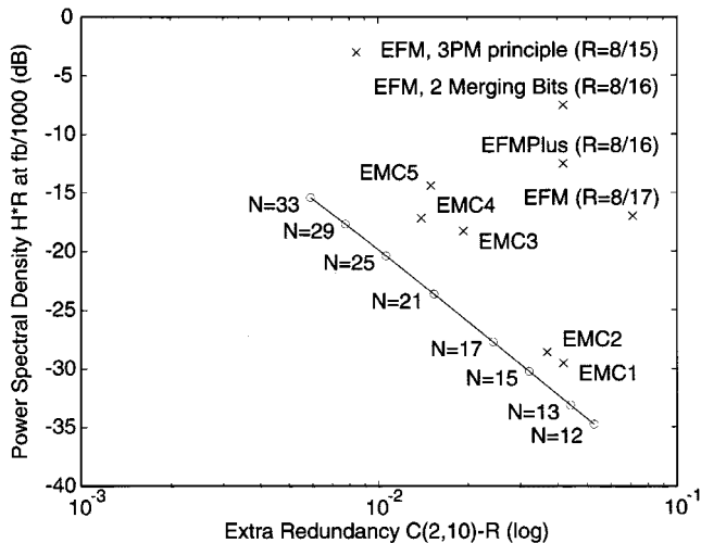
Fig. 4. Comparison of the performance of several (2, 10, 15) constrained modulation codes.
