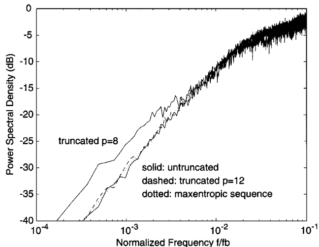
Fig. 3. Power spectra of several (2, 10, 15) constrained enumerative codes having a rate of 256/512 (obtained in computer simulations; solid, dashed) and power spectrum of the corresponding maxentropic sequence (evaluated using the method developed by Kerpez et al. [9], denoted by the dotted line).
