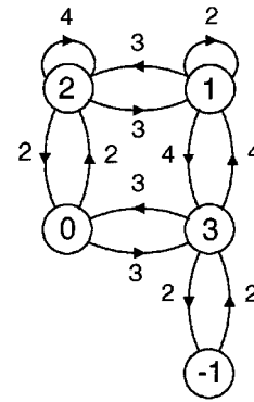
Fig. 1. Runlength graph representing the (1, 3, 7) constraint. The states are denoted by their U_j values, and the edges are labeled by their lengths [9].
